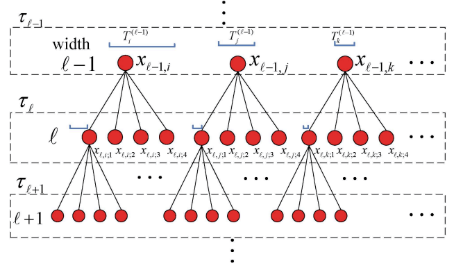
Fig. 1: Depiction of the layers of the trees, with n_c = 4 children considered. Note that each parent coefficient at layer \ell - 1 has a relative width T_i^{(\ell-1)} , and all widths at a given layer sum to one. The width of the parent is partitioned into windows of width T_i^{(\ell-1)}/n_c for the children.
