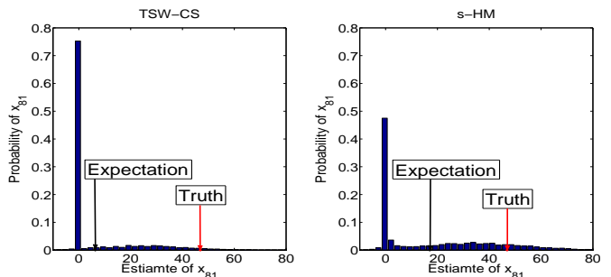
Fig. 3: Distribution of estimated x_{81} by proposed s-HM model (right) and TSW-CS (left).
