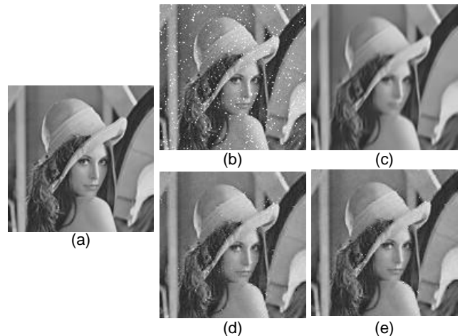
Fig. 6: Denoising. (a) original image, (b) noisy image (PSNR: 19.11dB), (c) dHBP (PSNR: 30.31dB), (d) shrinkage prior without tree (PSNR: 29.18dB), and (e) s-HM (PSNR: 30.40dB).
