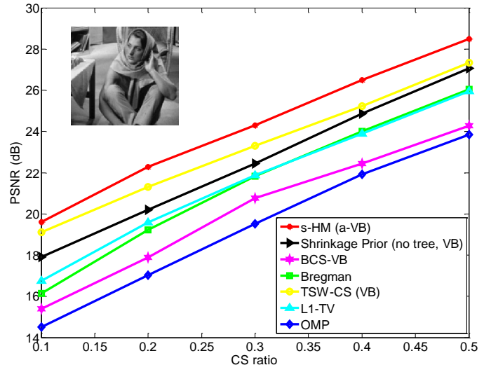
Fig. 2: PSNR comparison of various algorithms for compressive sensing with wavelet-based image representation.
