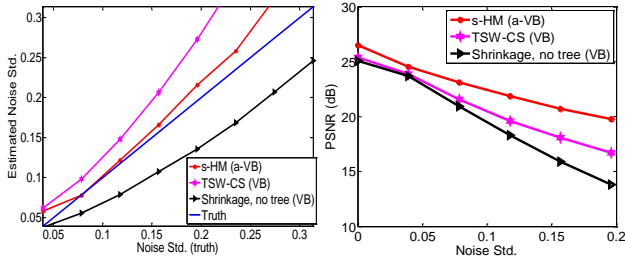
Fig. 4: Left: inferred noise standard deviation plotted versus truth. Right: reconstructed PSNR of “Barbara” with different algorithms, at CS ratio = 0.4 under various noise levels.
