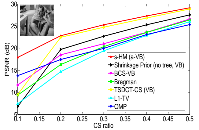
Fig. 5: PSNR comparison of various algorithms for compressive sensing with block-DCT image representation. The “TSDCT-CS” is the model implemented in [17], while the “s-HM” denotes proposed model with block-DCT tree structure, and “Shrinkage Prior (no tree)” symbolizes the flat model without tree-structure.
